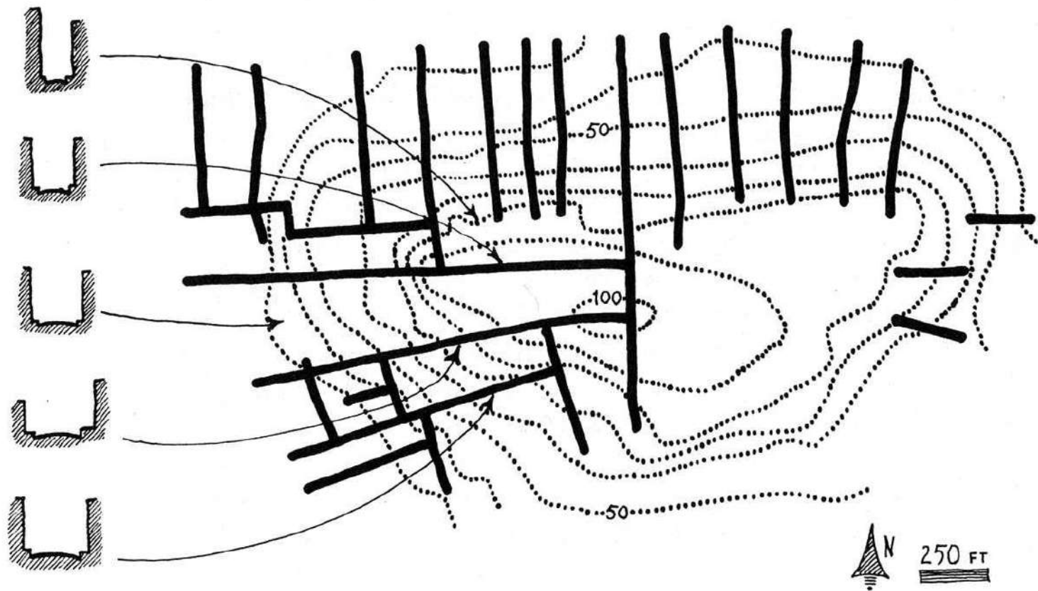
FIG. 51. Steep streets, topography, and street cross sections
